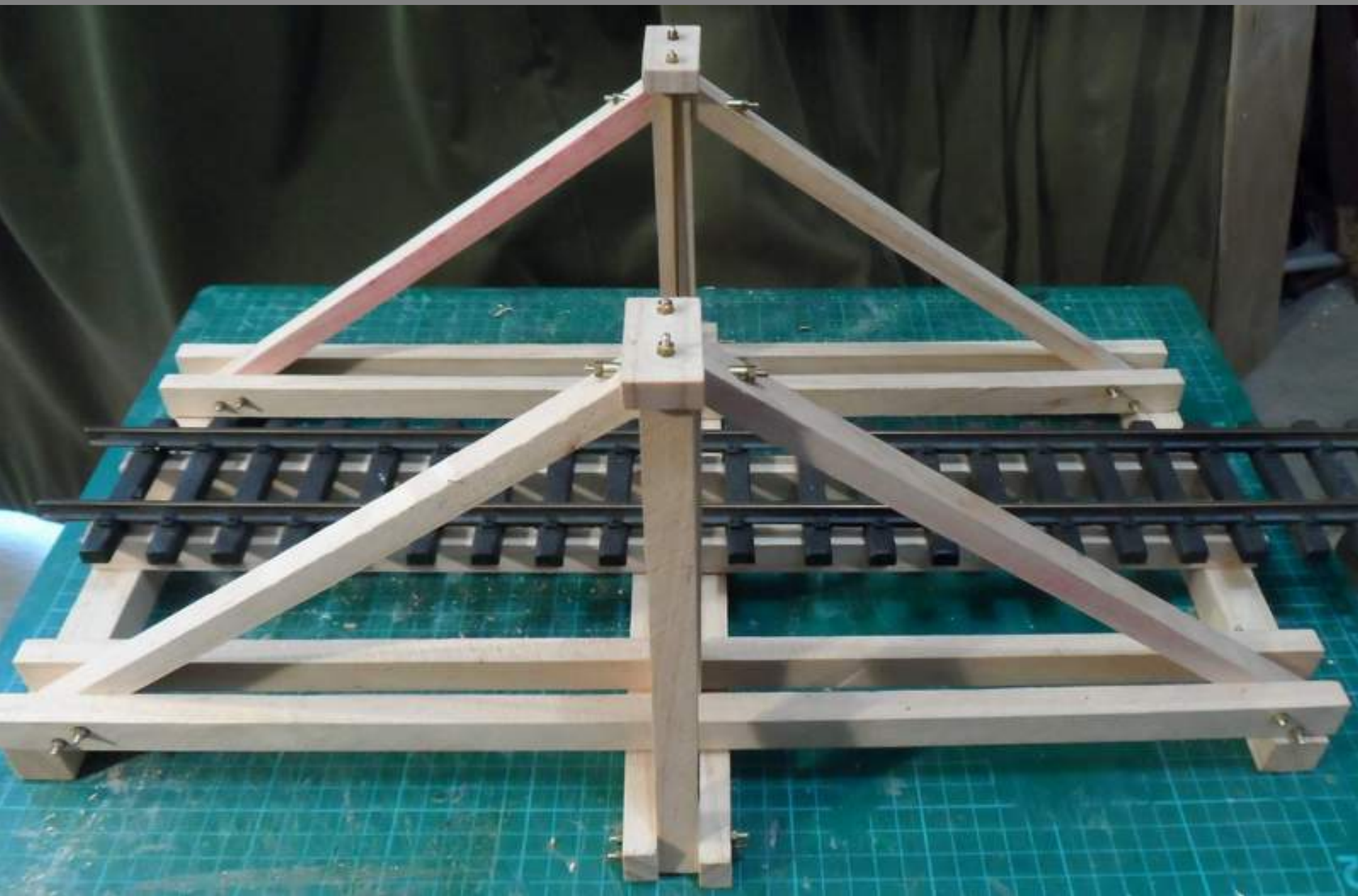
All Braces & Rods Fitted
